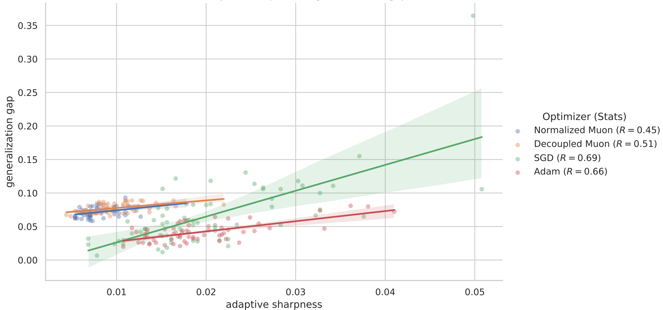
Correlation: adaptive sharpness vs generalization gap
